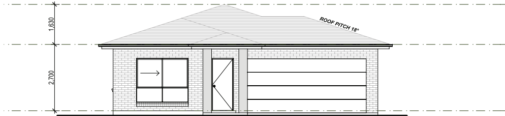
○ FRONT ELEVATION 1:100
